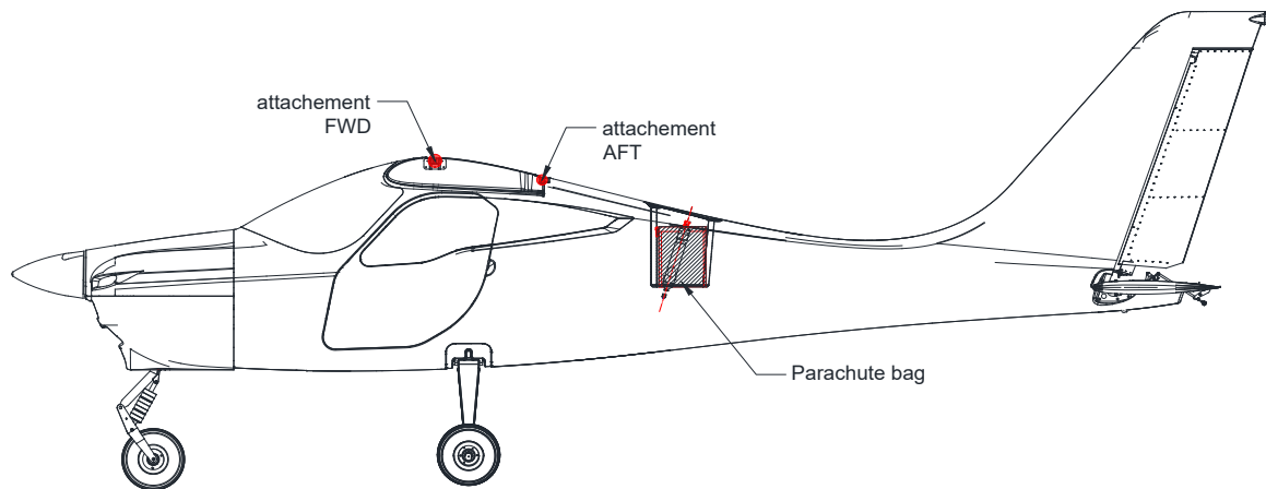
Fig. 7-16. P92 Echo MkII Rescue system
