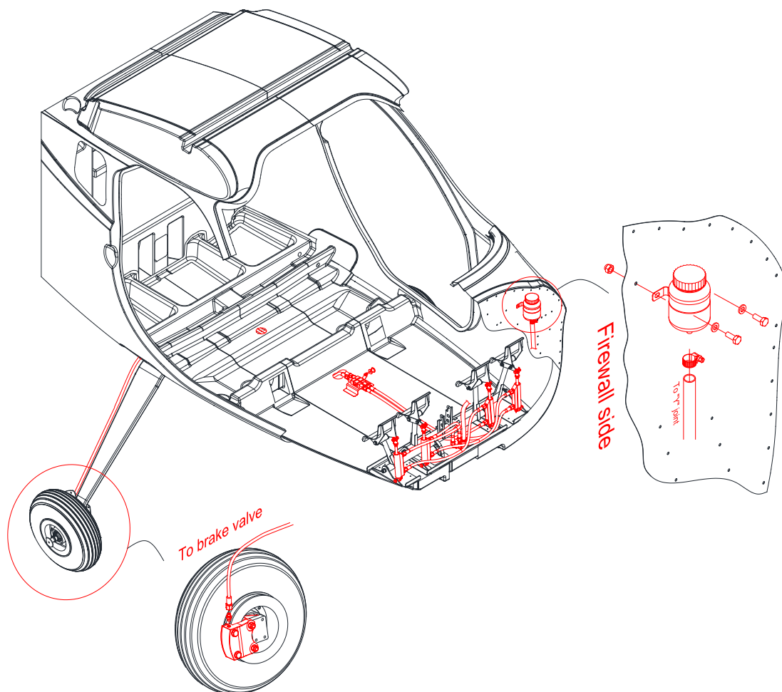
Fig. 7-11. P92 Echo MkII Brake System
