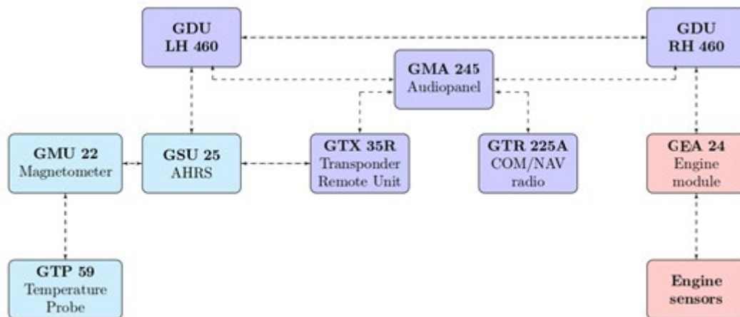
Fig. 7-12. Avionic Scheme
