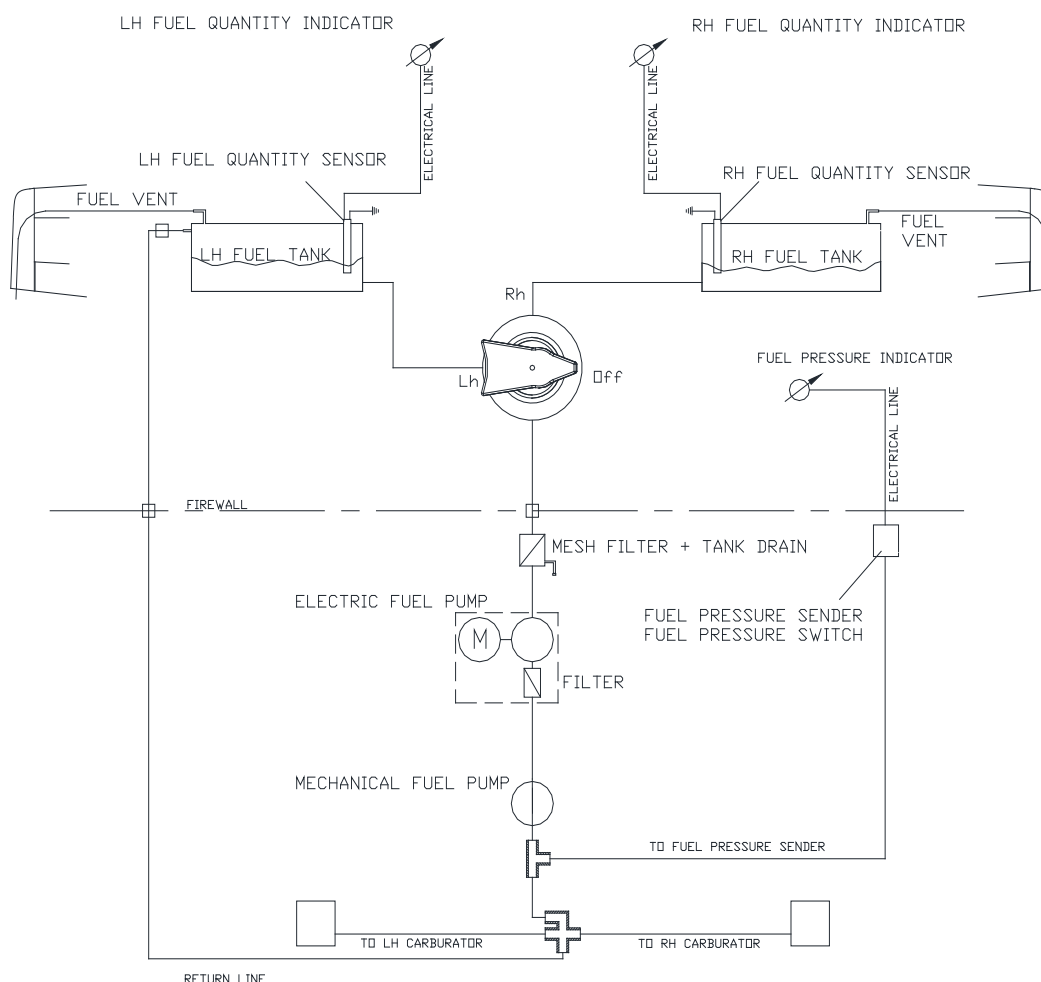
Fig. 7-15. Fuel System
