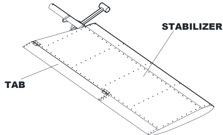
Fig. 7-3. P92 Echo MkII stabilator and tab
